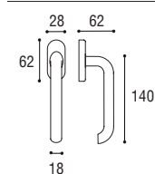
Maniglia per finestra DK \varnothing 7 x 40 Window handle DK \varnothing 7 x 40
