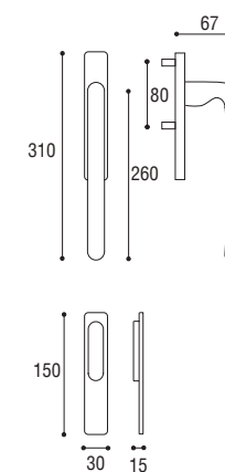
Maniglione singolo \varnothing 10 con conchiglia Single pull handle for sliding door \varnothing 10 with closed plate
