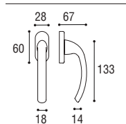
Maniglia per finestra DK \varnothing 7 x 40 Window handle DK \varnothing 7 x 40
